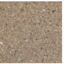
Landslide
